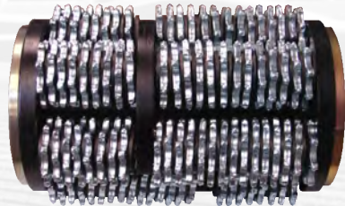
Hartmetalllamellentrommel carbide tipped cutter drum
